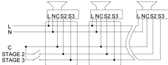
Fig 3 BExS110 AC Simplified Block Diagram
