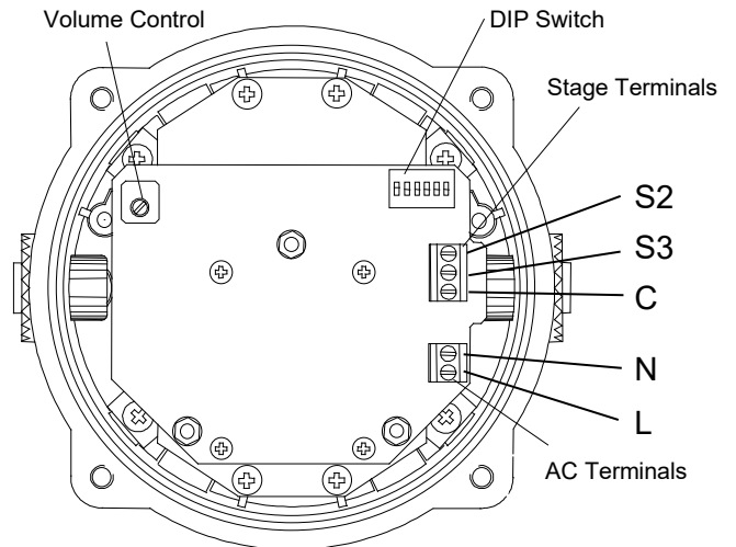
Fig. 4 AC Terminals
