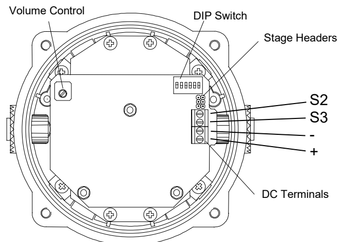
Fig. 6 DC Terminals
