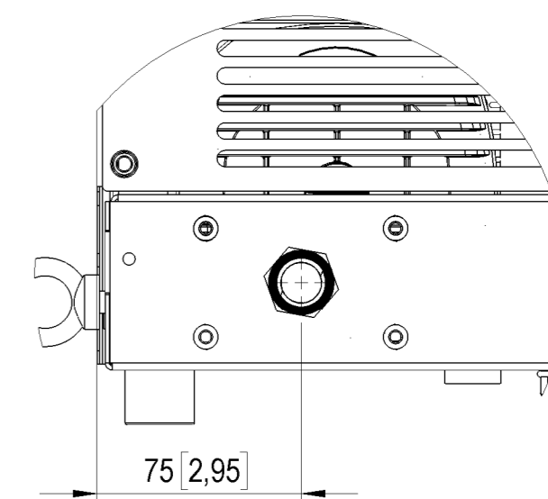
VIEW B SCALE 2 : 5
